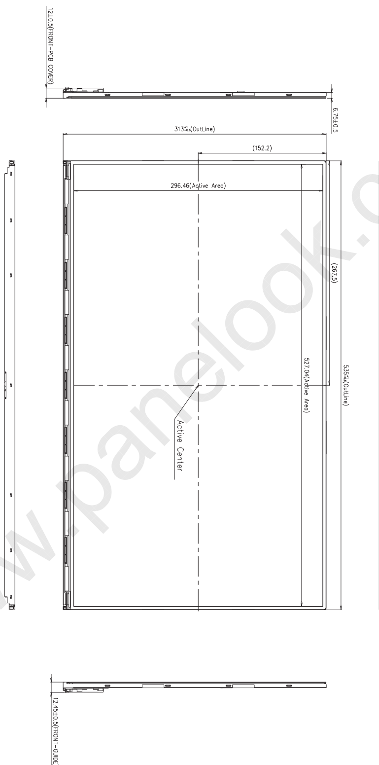
Figure 5. TFT-LCD Module Outline Dimensions (Front view)
